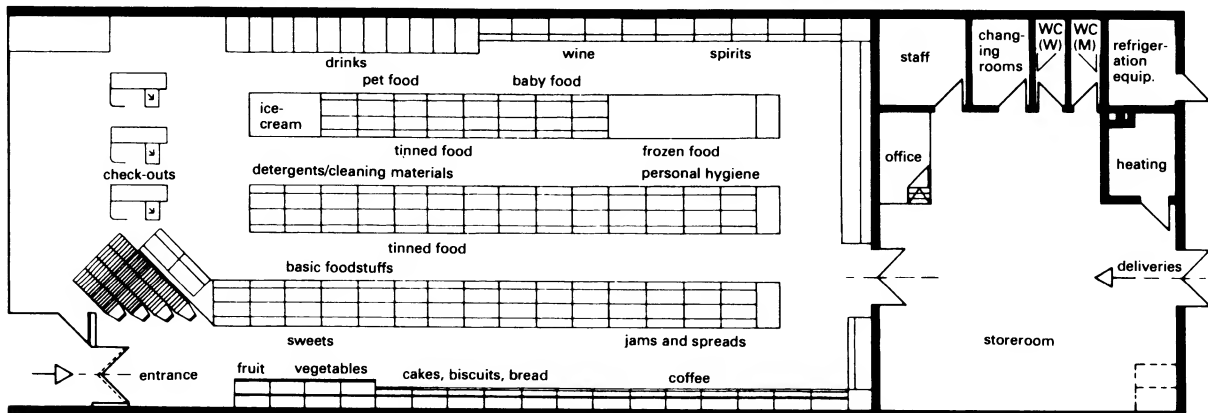
⑥ Discount market, 300–500m 2 sales area
